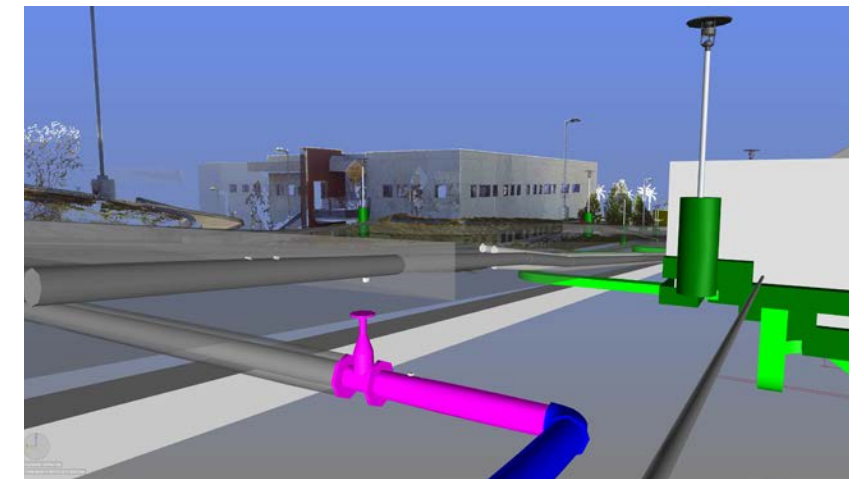
Composite Laser Scan and Utility Model
